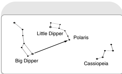
Fig. 50: Locating Polaris
