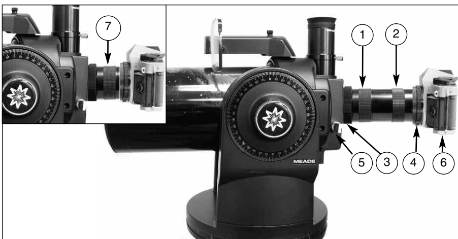
Fig. 30: Example of photography through the ETX using the #64 T-Adapter: (1) Short section of #64 T-Adapter; (2) Extension section of #64 T-Adapter; (3) Knurled attachment ring; (4) T-mount; (5) Flip-mirror control in “up” position; (6) 35mm camera body; (7) Format 1.
