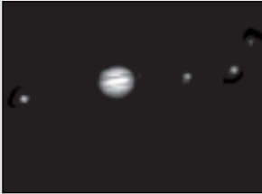
Fig. 58: The planet Jupiter. Jupiter's four largest moons can be observed in a different position every night.
