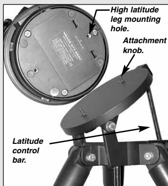
Fig. 45: High latitude leg mounting hole and corresponding attachment knob.
