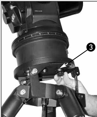
Fig. 46: Attach telescope to tripod.
