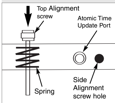
Fig. 55: Interior side view of LNT Module.
